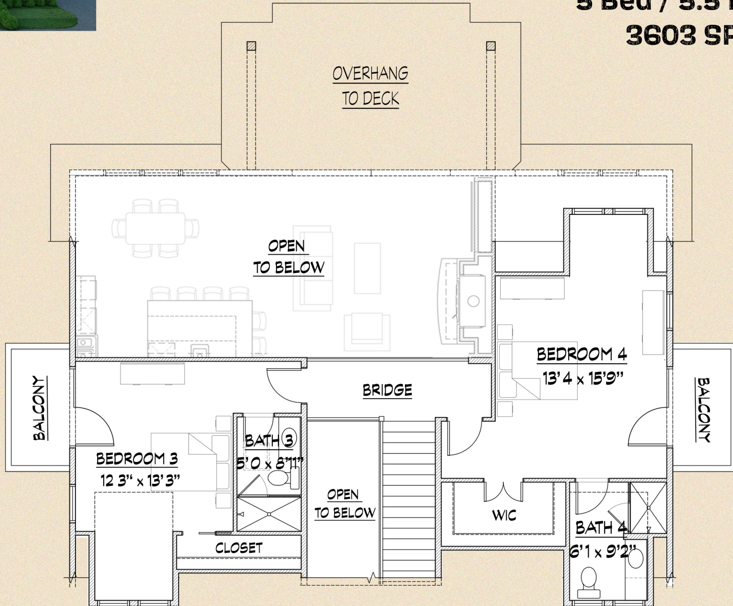
2 UPPER LEVEL FLOOR PLAN
