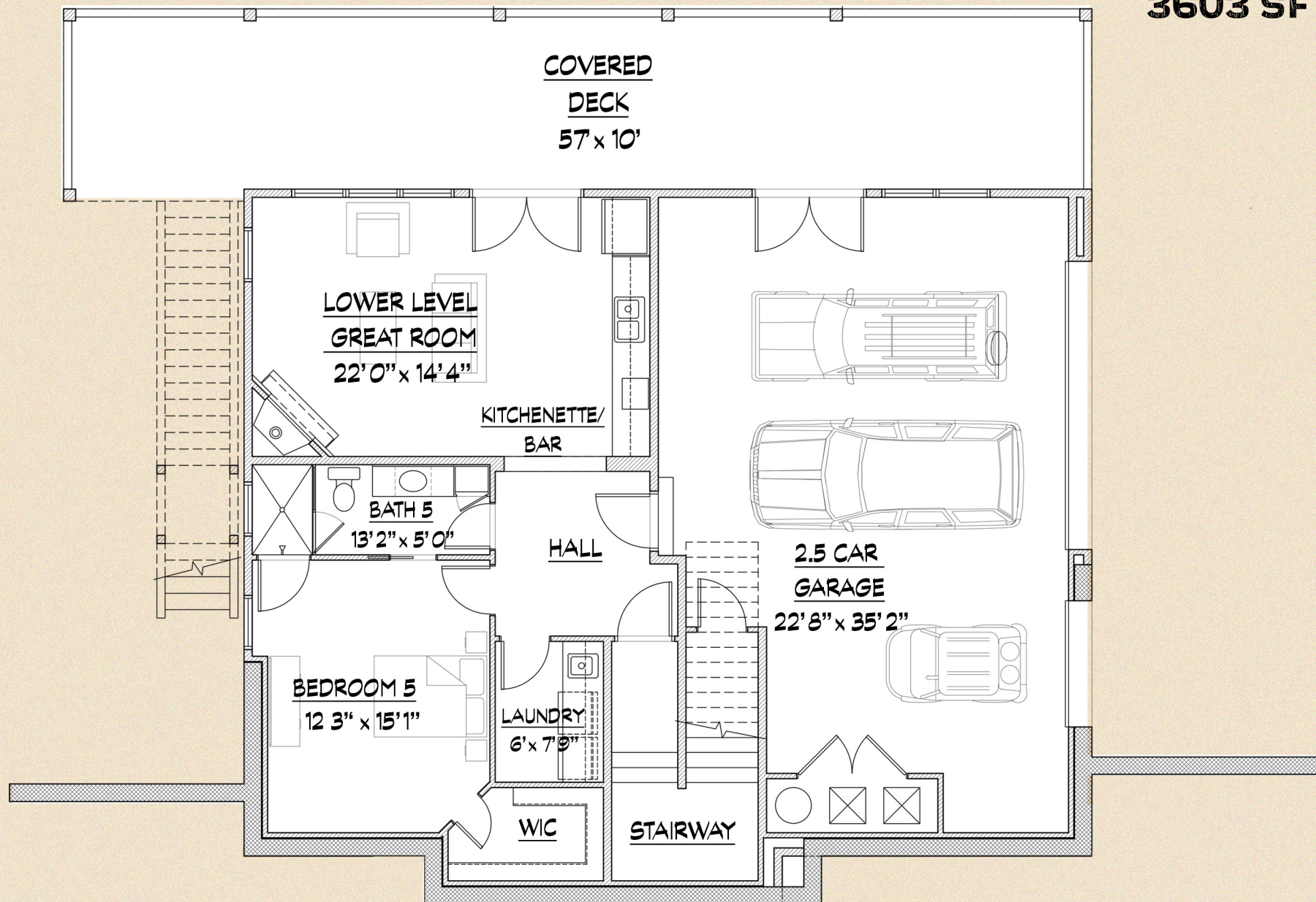
3 LOWER LEVEL FLOOR PLAN
