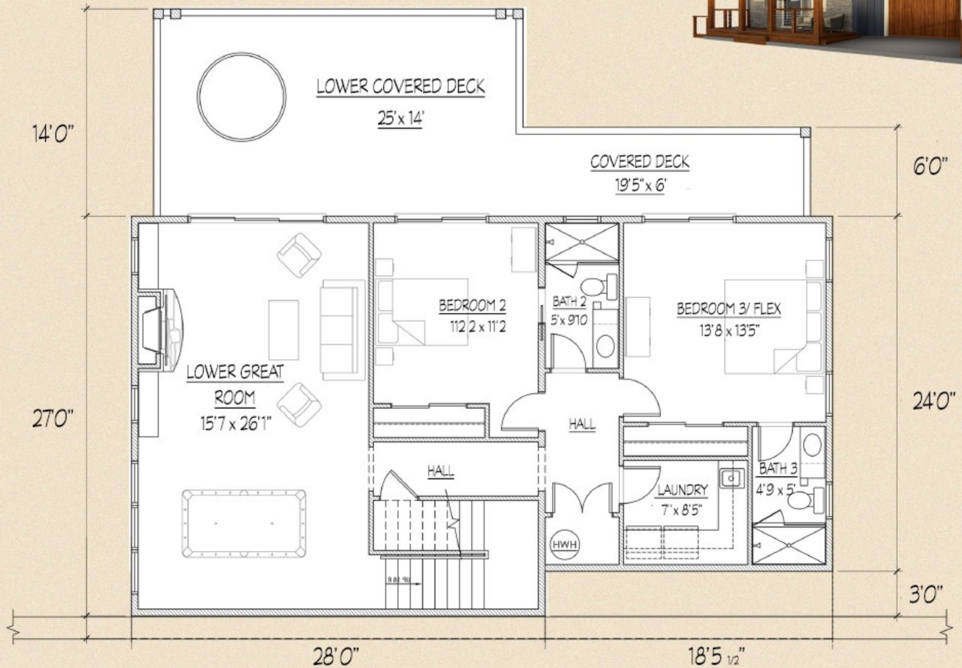
2 LOWER LEVEL FLOOR PLAN
