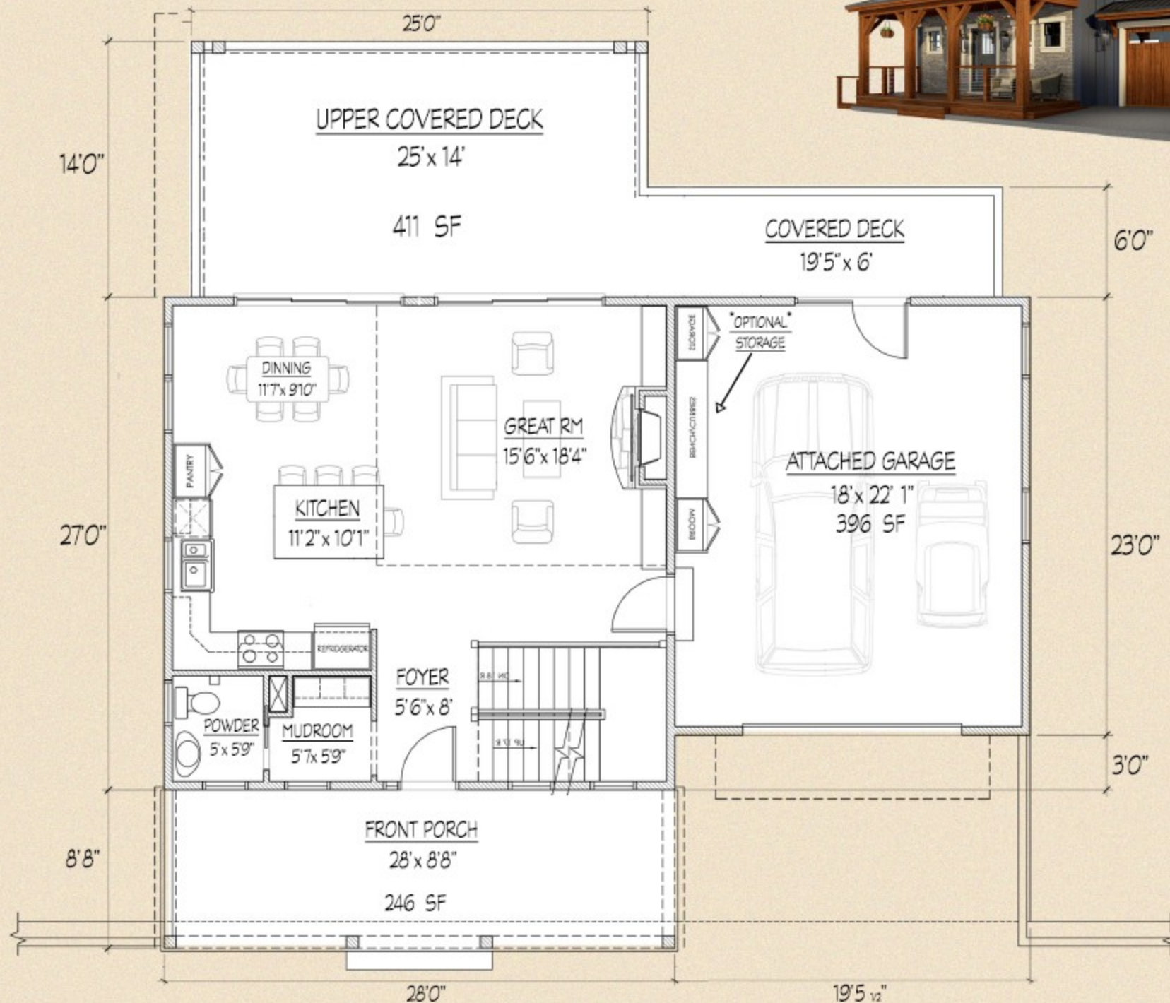
1 MAIN LEVEL FLOOR PLAN
