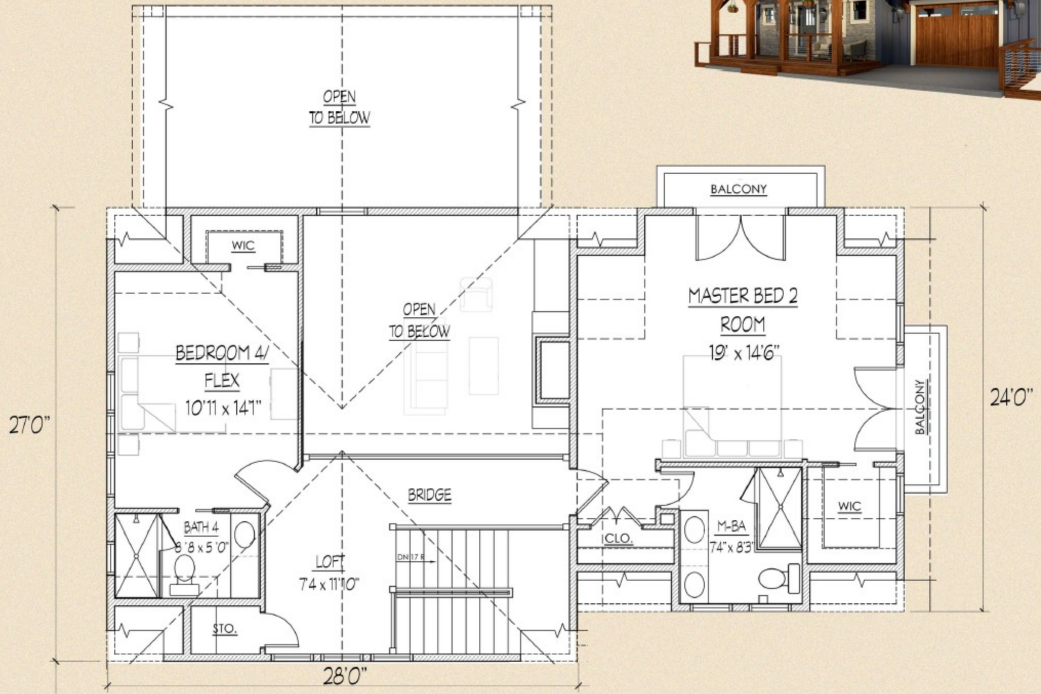
3 UPPER LEVEL FLOOR PLAN
