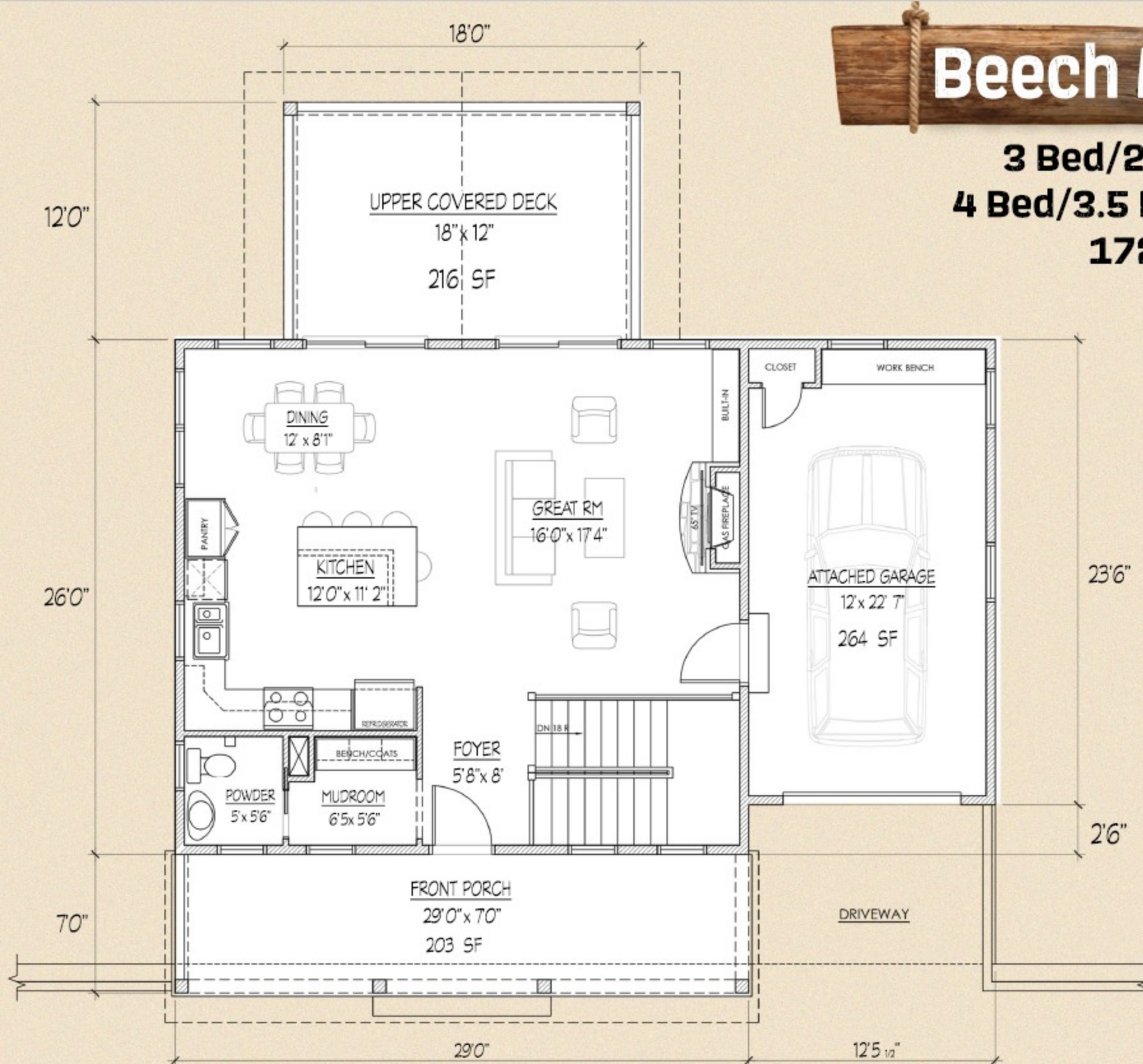
1 MAIN LEVEL FLOOR PLAN
