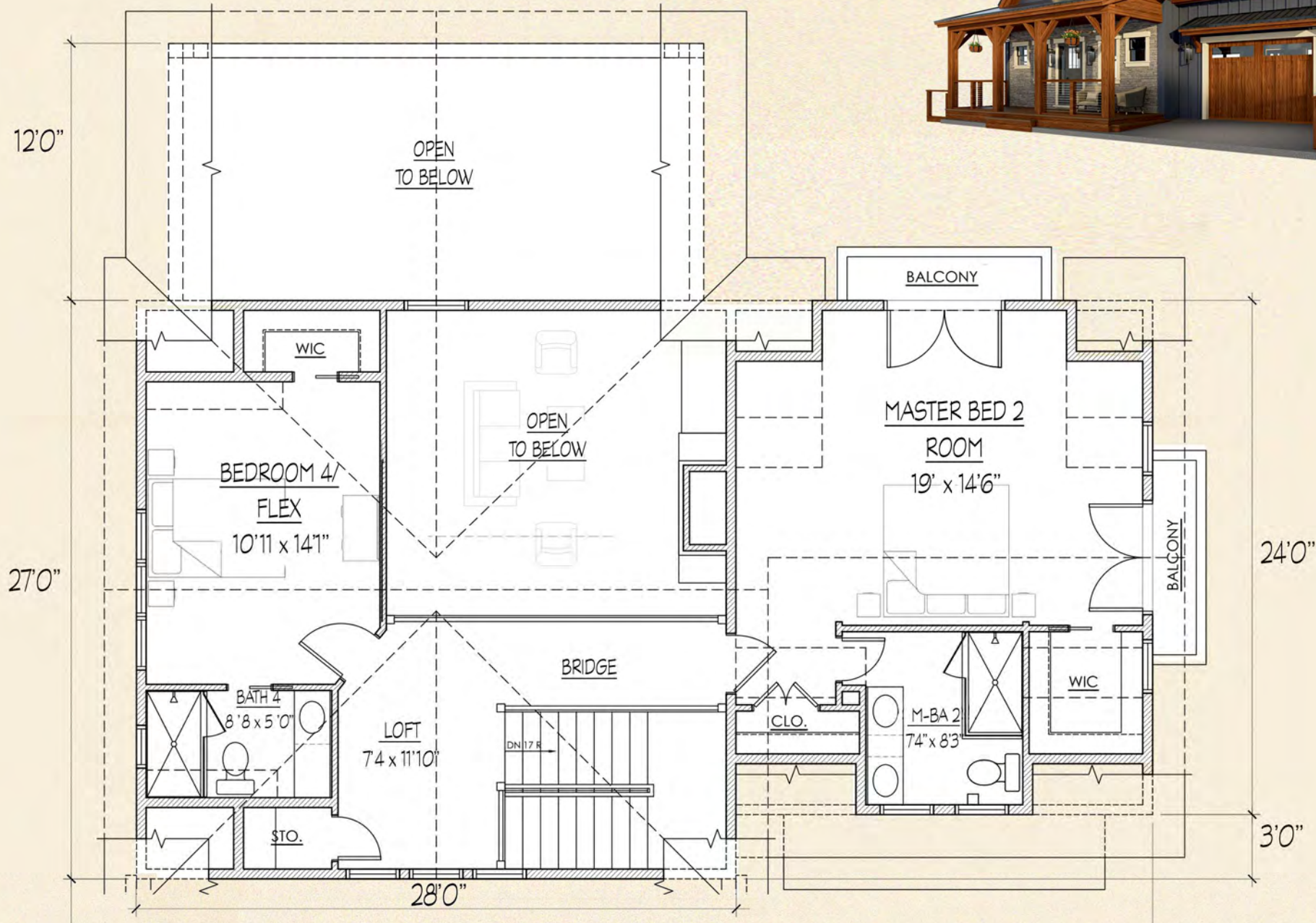
3 UPPER LEVEL FLOOR PLAN
